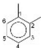
1,2-dimethylbenzene (ortho-xylene)
